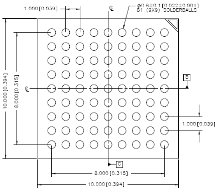
BGA Package Dimensions
